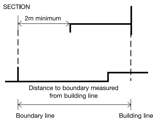
Diagram 21 The effect of a canopy on separation distance
